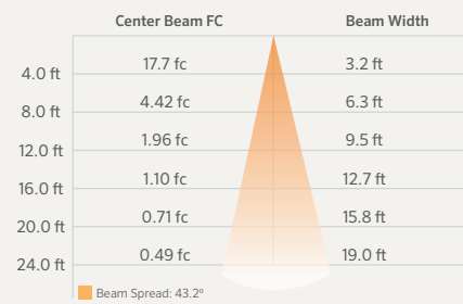
FC-ZDC 3LED (RG) ILLUMINANCE AT A DISTANCE
