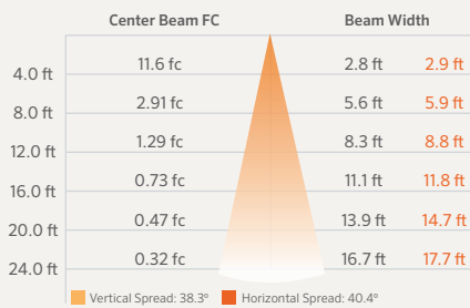
NP-ZDC 3LED ILLUMINANCE AT A DISTANCE
