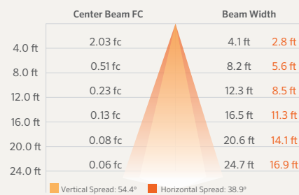
KG-ZDC 3LED ILLUMINANCE AT A DISTANCE
