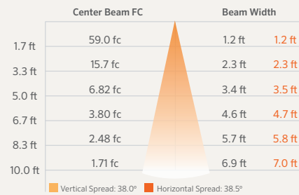
DE-ZDC 3LED ILLUMINANCE AT A DISTANCE
