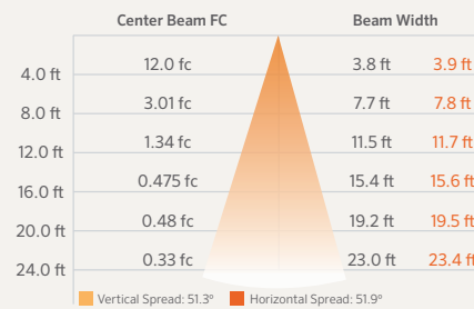
VS-ZDC 3LED ILLUMINANCE AT A DISTANCE
