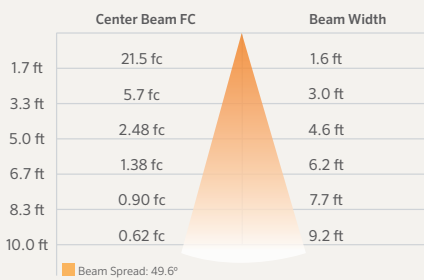
NL/PS-ZDC 3LED ILLUMINANCE AT A DISTANCE
