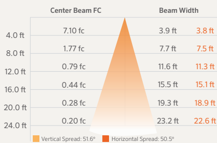
PE-ZDC 3LED ILLUMINANCE AT A DISTANCE
