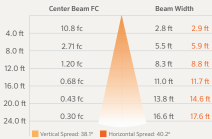
LC-ZDC 3LED ILLUMINANCE AT A DISTANCE
